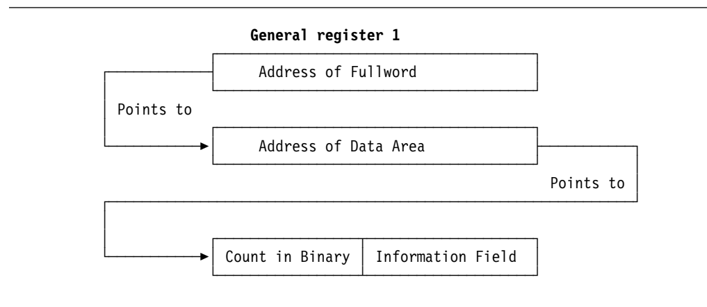
Figure 71. Access to PARM field
