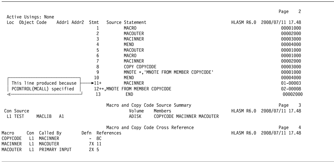
Figure 10. Assembly with LIBMAC and PCONTROL(MCALL) options
